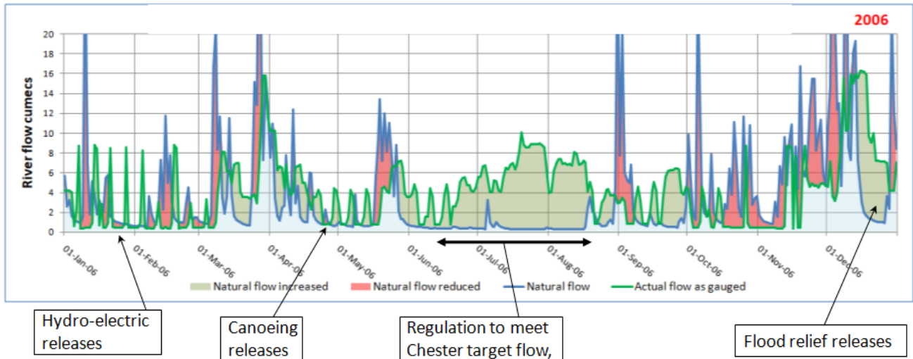
Figure 5 - Changes to flows due to regulation of up to 800 MI/d below Llyn Celyn dam
