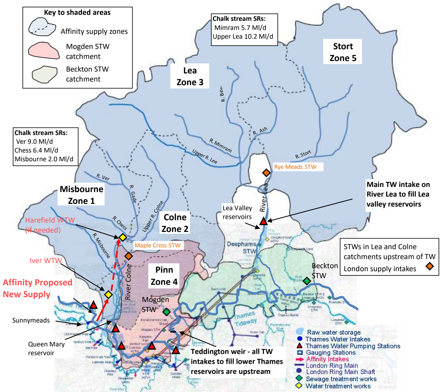
Figure 3-1 Affinity Central Region supply zones and drainage catchments
