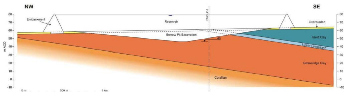
Figure K1 - Cross-section of reservoir showing borrow pit
