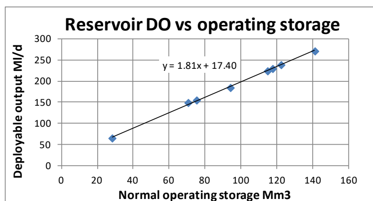
Figure K2 - Abingdon reservoir deployable output vs normal operating storage
